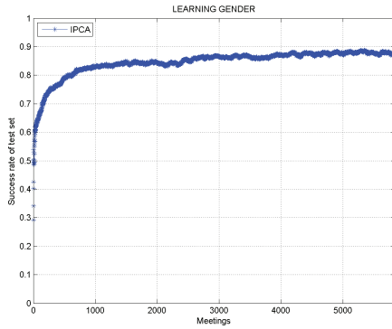
Fig. 3. Gender classification performance evolution testing the complete dataset of static images.
